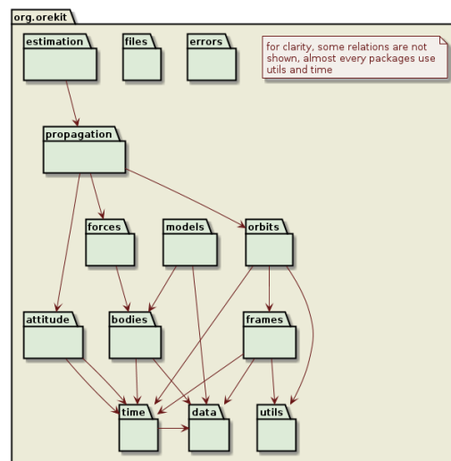
Figure 2. Orekit package structure. Source: [5]
